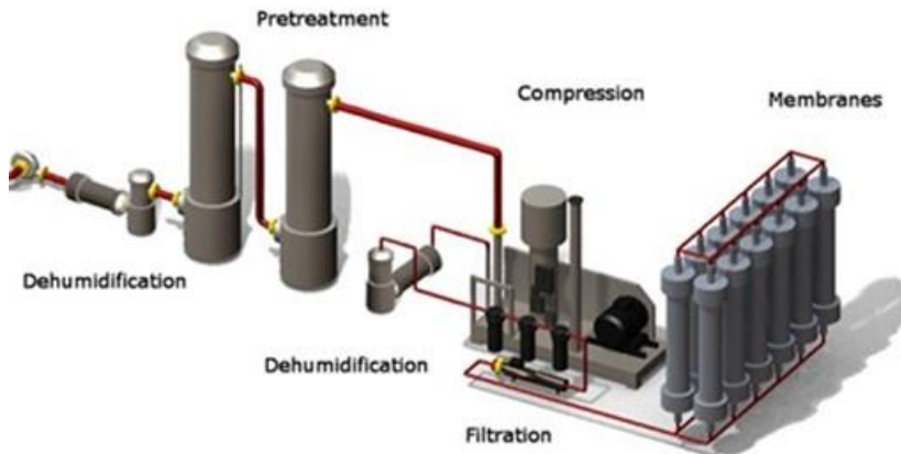
Biogas Upgrading
