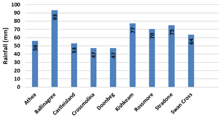
Cumulative Rainfall 01 to 30 of Apr
