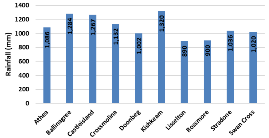
Cumulative Rainfall 2021
