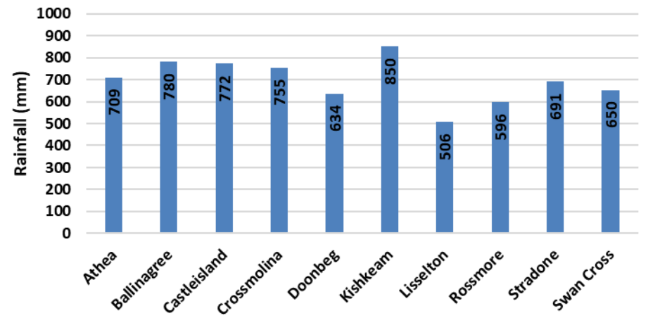
Cumulative Rainfall 2021
