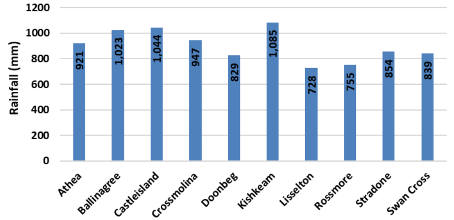
Cumulative Rainfall 2021
