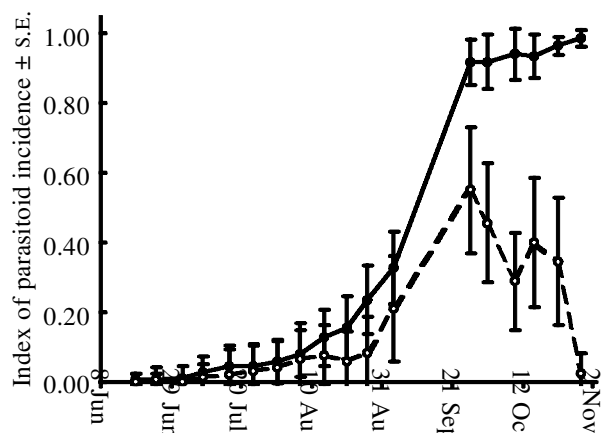
Fig. 2. Mean incidence of a) P. pilosus mummies (RPP index) and b) P. pilosus adults (RAI index) within the intensively sampled grid following the release of parasitoids at site (KM1).
