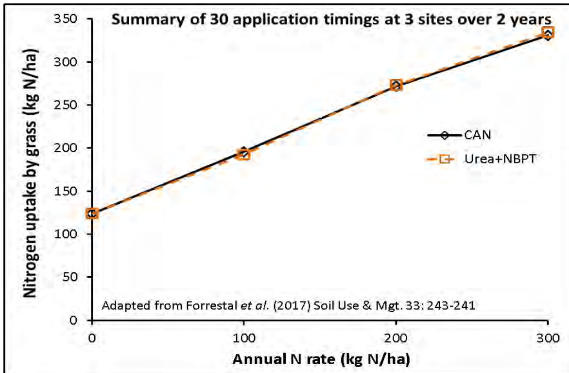
Figure 3. Summary of N recovery (off take kg/ha N) for CAN and protected urea evaluated on 30 occasions (application timings) conducted across the growing season on three soils over two years.
