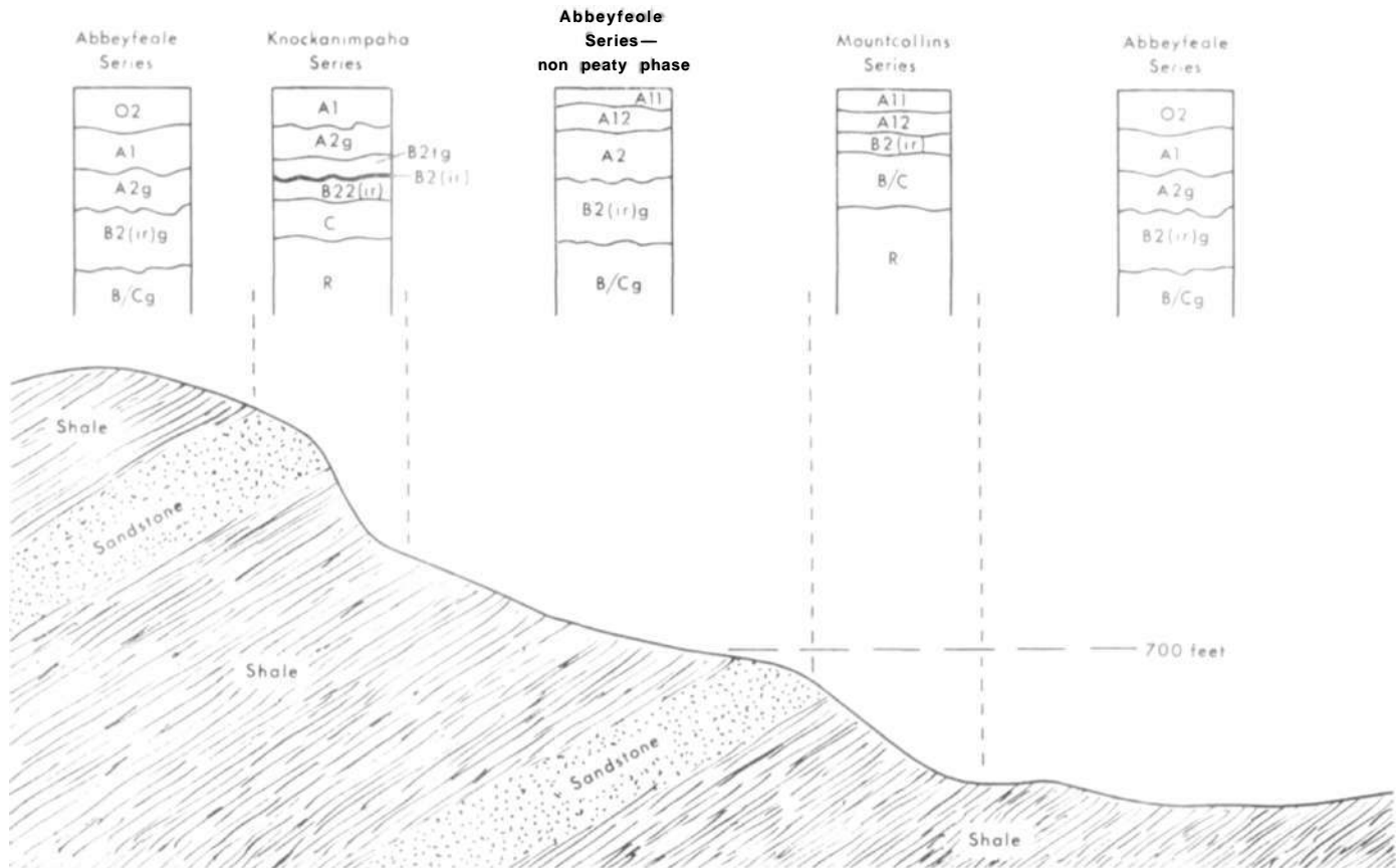
Fig. 4: Abbeyfeale and associated soils in relation to topography and geology (vertical s v/
