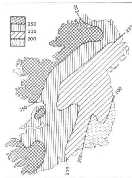
Fig. 4: Average number of raindays per year.
