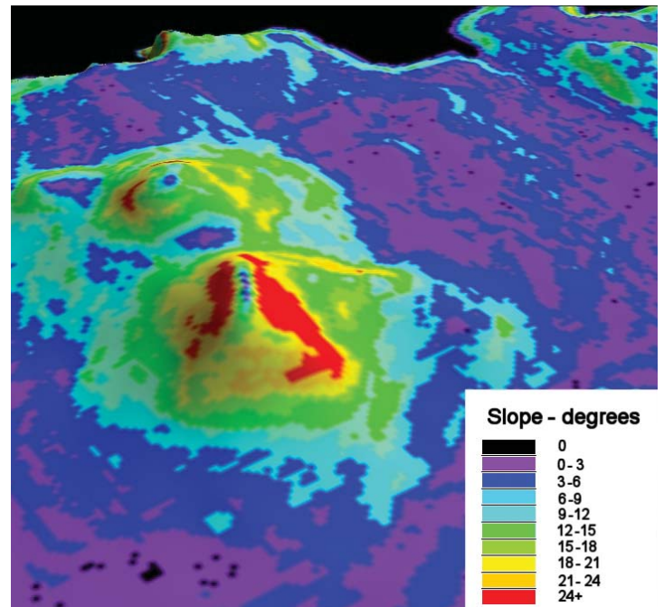
Belderg slope model. Belderg, North County Mayo: colour-coded slope map 'draped' over corresponding elevation model. One example of physiographic landscape features that can be used in predictive soil mapping.
