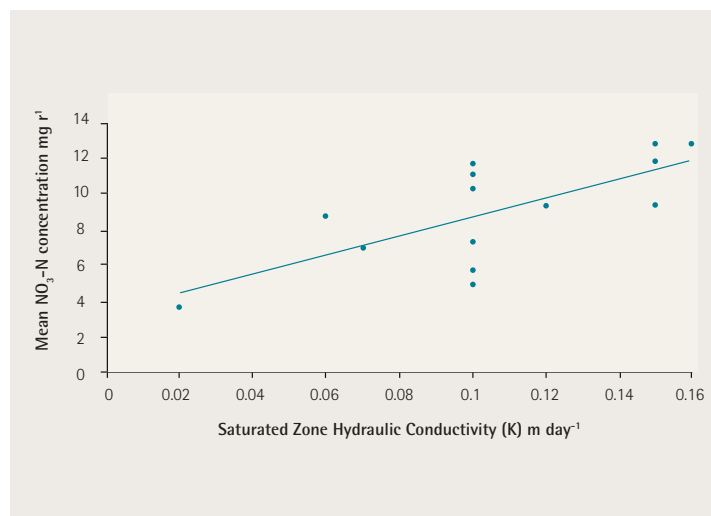
FIGURE 2: The positive relationship ( p=0.003 ) between groundwater \text{NO}_3^- and the speed of groundwater movement (saturated zone hydraulic conductivity, K_{SAT} ) (Fenton et al. 2009).
