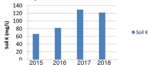
Figure 3: soil K
