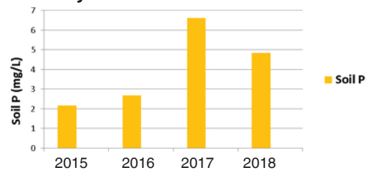
Figure 2: soil P
