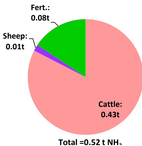
Figure 83: Total Ammonia Emissions for the average Tillage Farm
