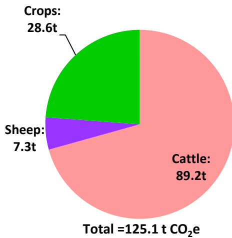
Figure 82: Agricultural GHG Emissions for the average Tillage Farm
