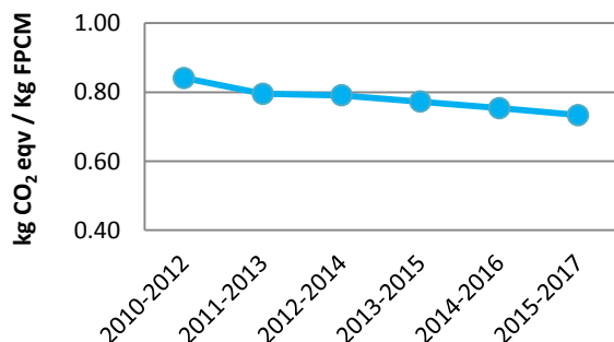
Figure 120: Ag. GHG Emissions per kg FPCM: 2012-2017 (IPCC approach) 3 year rolling average – Dairy Farms
