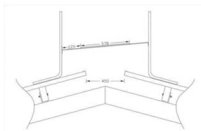
Figure 3: Protected ridge with upstands
