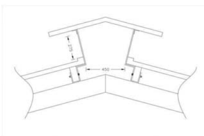
Figure 3: Protected ridge with upstands
