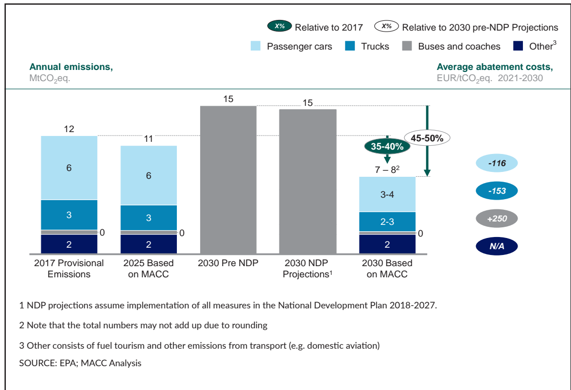
Figure 10.1 Annual Emissions and Average Abatement Costs in Transport
