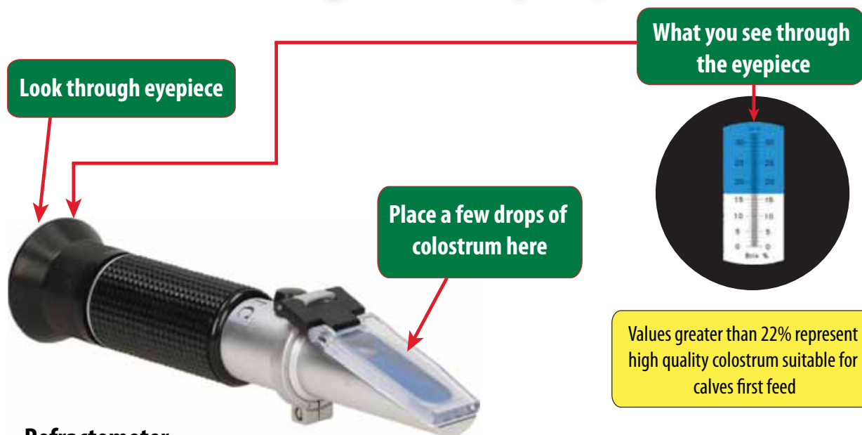
Refractometer
