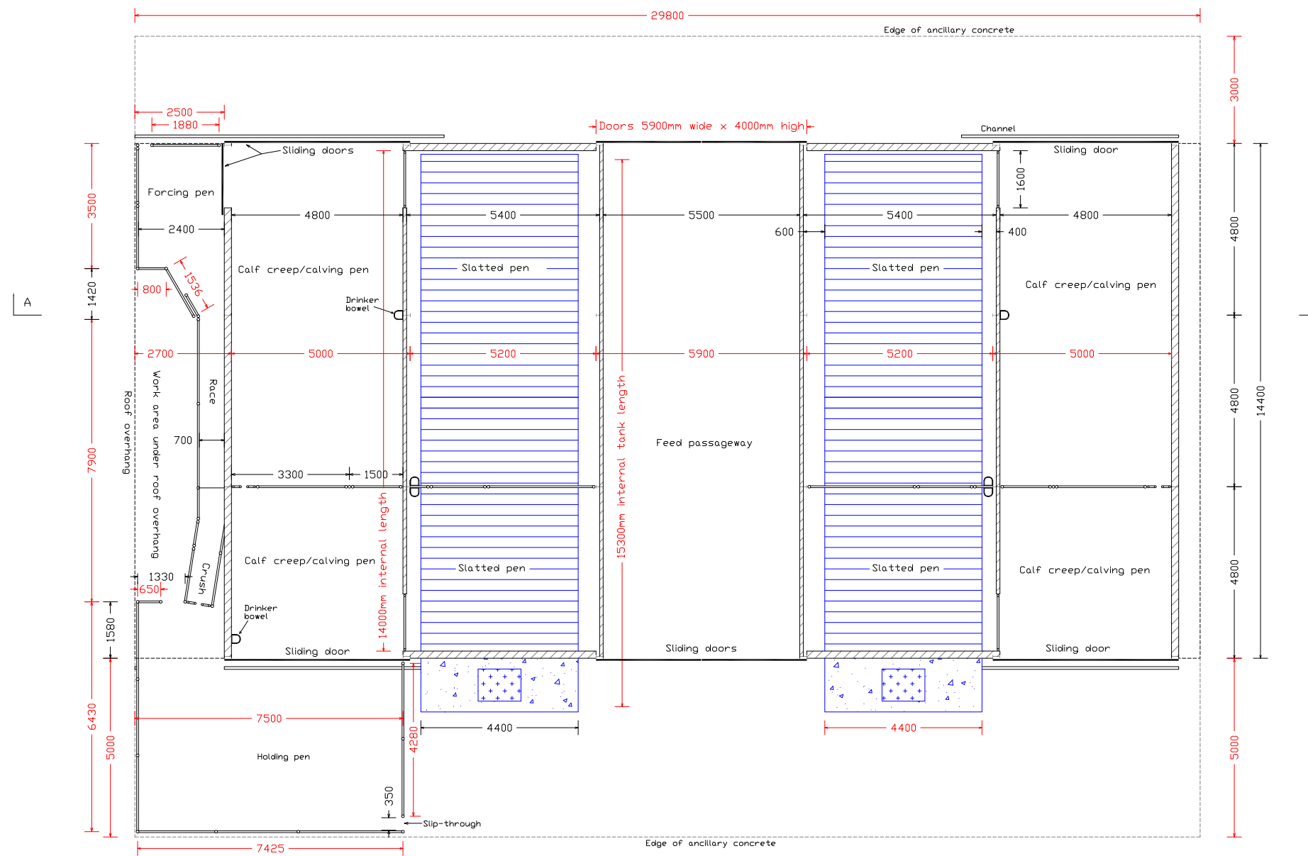
Slatted suckler unit with creep/calving pens and handling facilities
