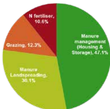
Figure 5. Breakdown of sources of NH 3 emissions in Ireland
