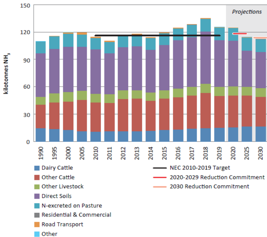
Figure 6. Trends in NH 3 emissions between 1990 and 2019 with projections to 2030
